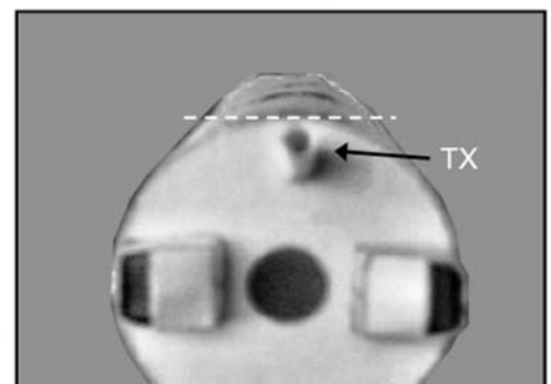
Glue TX in to a tube. Then glue TX to the small circle on the rockets base. Align it so that the seam is directly toward the center, while the vent is facing directly outward and away from the center.
