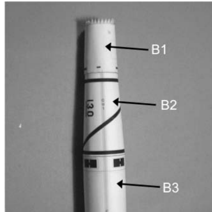
Glue B2 to B3, and then B1 to B2. Use a small rod to roll the conduit parts CL and CU into
